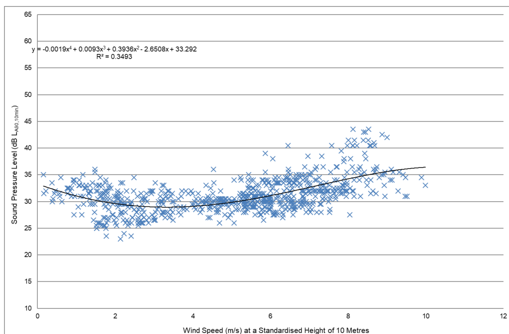
Figure A12-3-3 Baseline Noise Levels L_{A90, 10 \text{ min}} dB – Location B – Daytime Period
