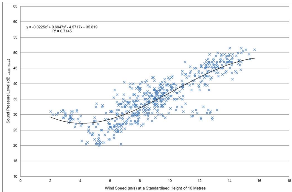
Figure A12-3-1 Baseline Noise Levels LA90, 10 min dB – Location A – Daytime Period
