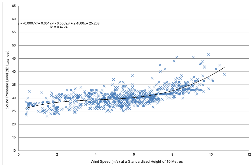
Figure A12-3-4 Baseline Noise Levels L A90, 10 min dB – Location B – Night Time
