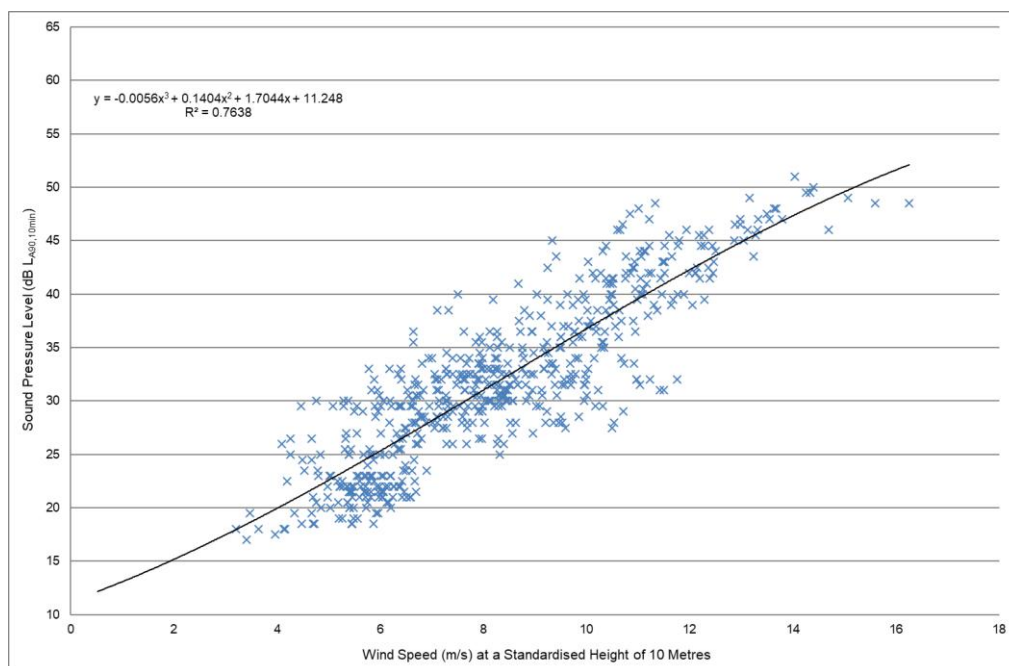
Figure A12-3-2 Baseline Noise Levels L_{A90, 10 \text{ min}} dB – Location A – Night Time
